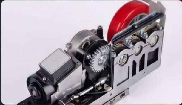
Precision Gear Mechanism — Reinforced steel drive for consistent, heavy-duty performance
